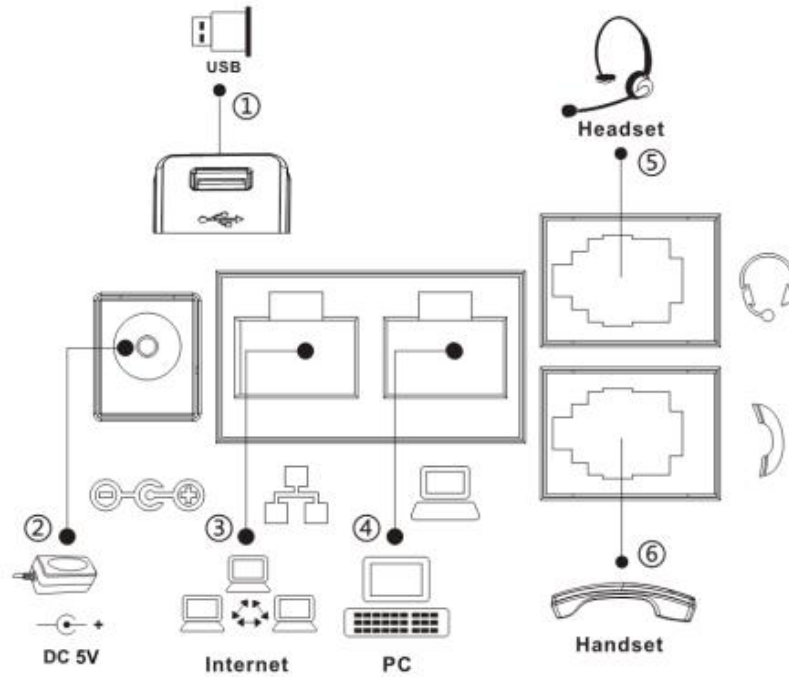
Picture 3 - Connecting to the Device of J4SG
