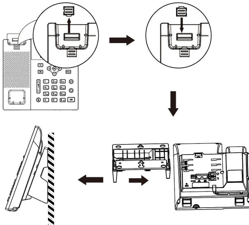
Picture 2 - Wall-mounted installation of J4SG
