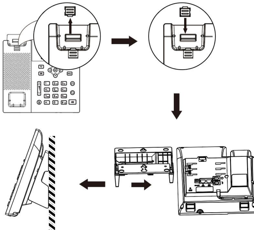
Picture 2 - Wall-mounted installation of J3SG
