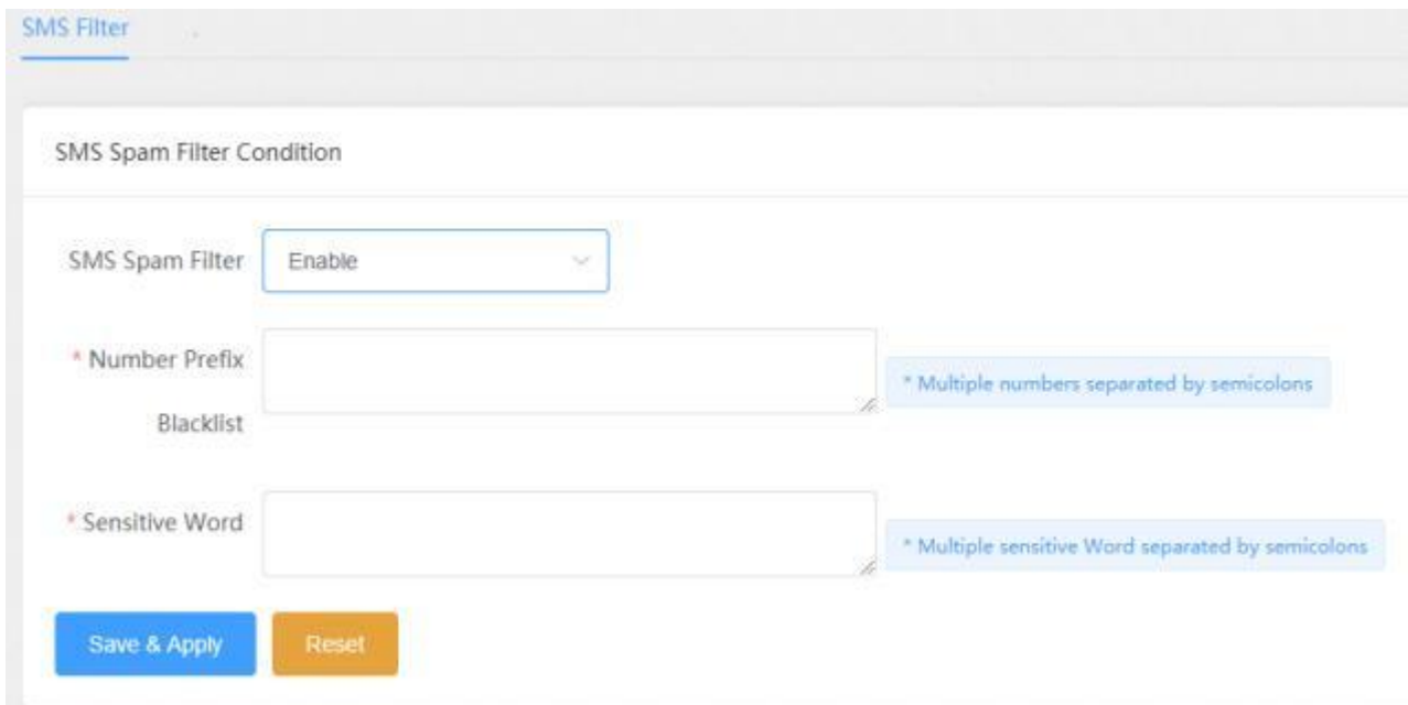
Figure 3.4.8-1 SMS spam filter
